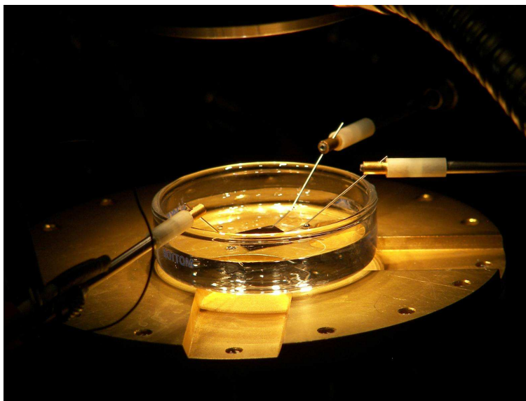
Figure 3.4: Photo of dielectrophoresis apparatus. Dielectrophoresis is performed by placing the die in a beaker of water and driving an electrical field on the driving pads through the micromanipulators shown.
