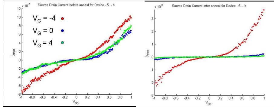
Figure 4.5: Effect on the electrical properties from annealing in vacuum at 100^{\circ}\text{C} overnight. The resistance of the devices increases substantially but the devices are much more sensitive to a gate voltage.
