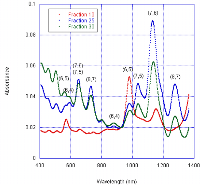
Figure 4.1: Absorption Measurement of 3 different fractions of purified carbon nanotubes. Fraction 10 is predominantly (6,5) chirality while the other fractions have a larger mix of carbon nanotubes.
